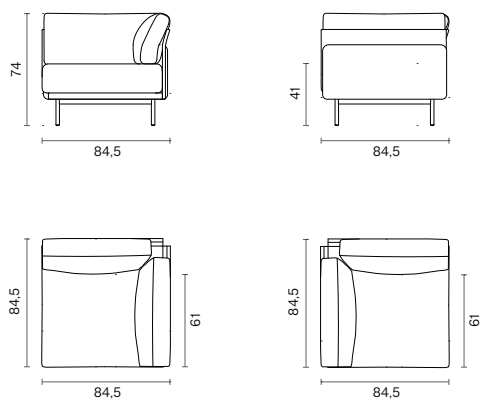
84,5 CORNER - 84,5C
