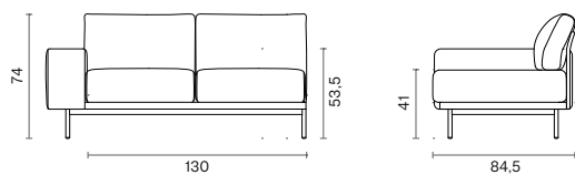
155 RIGHT - 155R
