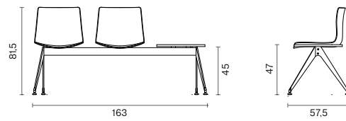
DOUBLE SEATS WITH LEFT TABLE
