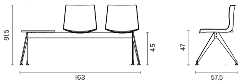
DOUBLE SEATS WITH RIGHT TABLE
