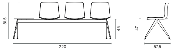
TRIPLE SEATS WITH RIGHT TABLE
